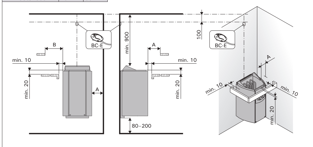
Figure 6. Safety distances (all dimensions in millimeters)
